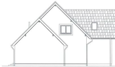
West elevation 1:100
